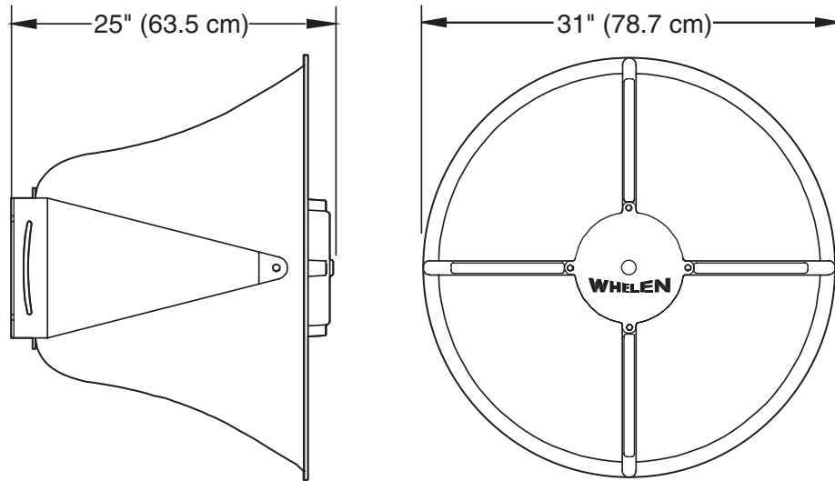
WS400H Speaker with standard wall mounting bracket
